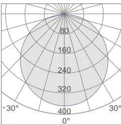
T5-4J16 120° Photometric
