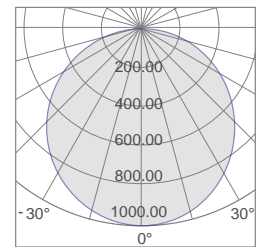
TPL-4E36 Photometric
