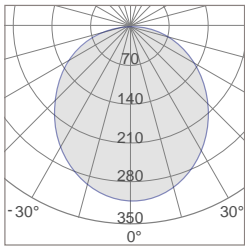
TPL-2HE30 Photometric
