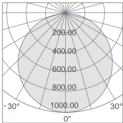
TPL-4HB40 Photometric
