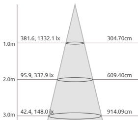
PLS-6060 Luminance
