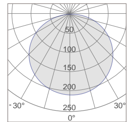
TPL-4HT40 Photometric
