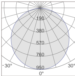
TPL-4HC40 Photometric
