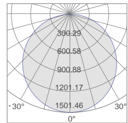
WPR-4B40 Photometric
