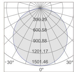
TPL-4D36 Photometric
