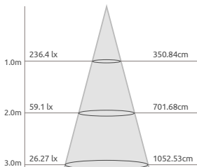
TPL-2HE30 Luminance
