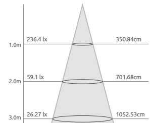
TPL-4HN40 Luminance
