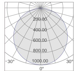
TPL-4HN40 Photometric
