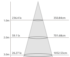
B6-RB Luminance
