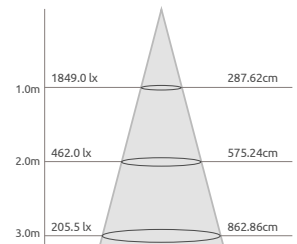
TPL-4F10 Luminance
