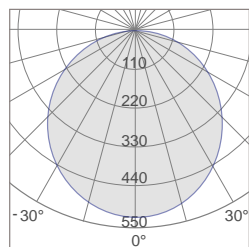
TPL-2JA18 Photometric
