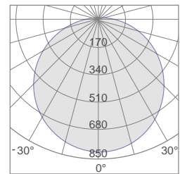
TPL-2J270 Photometric
