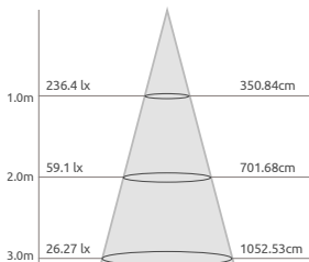
TPL-4HB40 Luminance
