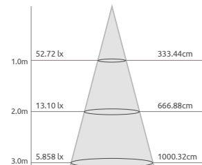
TPL-4HT40 Luminance
