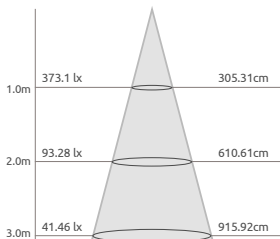
T5-4J16 120° Luminance
