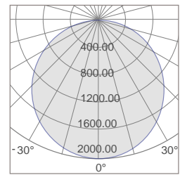
TPL-4F10 Photometric
