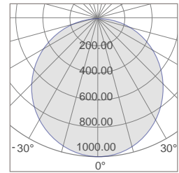
B6-RB Photometric
