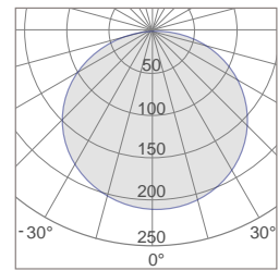
XDD-HA15 Photometric
