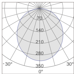
TPL-4IA40 Photometric
