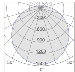
TPL-4H40 Photometric
