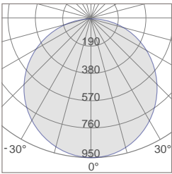
TPL-2C18 Photometric
