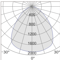
90° Photometric
