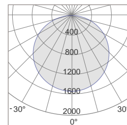
3060H 110° Photometric
