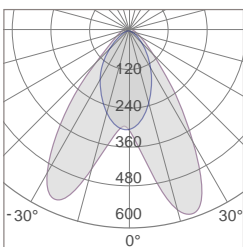
PLD-1358I Photometric
