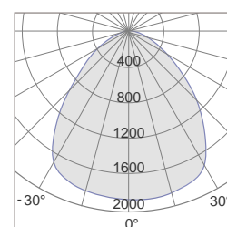
90° Photometric
