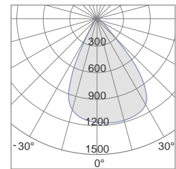
90° Photometric
