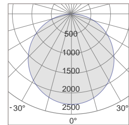
PLS-6060 110° Photometric
