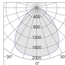
110° Photometric
