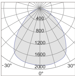
90° Photometric
