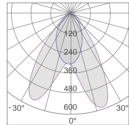
PLD-1358K Photometric
