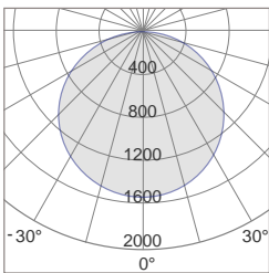
3060H 110° Photometric
