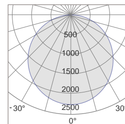
110° Photometric
