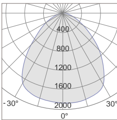
90° Photometric
