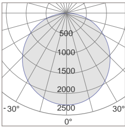
110° Photometric
