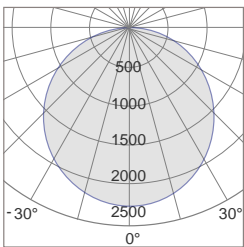
PLS-6060 110° Photometric
