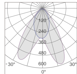
PLD-1358G Photometric
